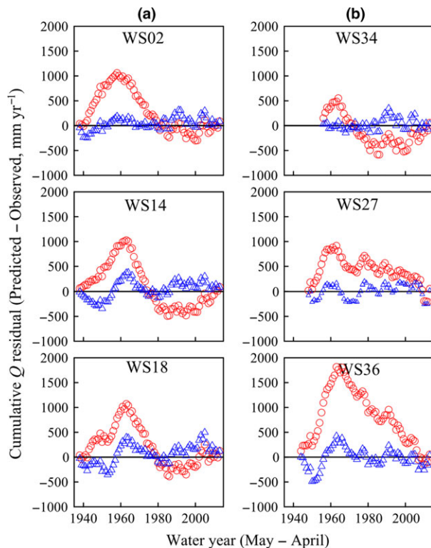
Fig. 5 Cumulative Q residuals (predicted–observed) for low-elevation (a) and high-elevation (b) watersheds (WS). Red circles are the cumulative residuals using models that predict Q as a function of climate only (model 9 Table 3b). Blue triangles are cumulative residuals using models that also include interventions (Climate and forest structure and species composition models in Table 5). Interventions added to the models minimized the relationship between residuals and water year as indicated by the white noise statistical test for residuals in Table S6, and represent changes in Q due to changes in forest structure and species composition.
